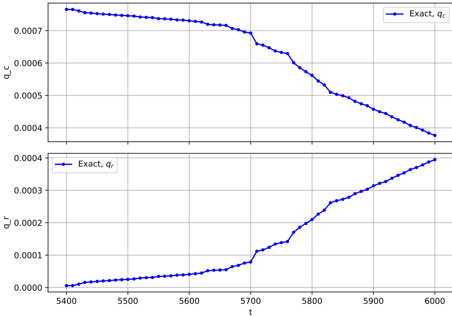
Trajectory No. 2387
