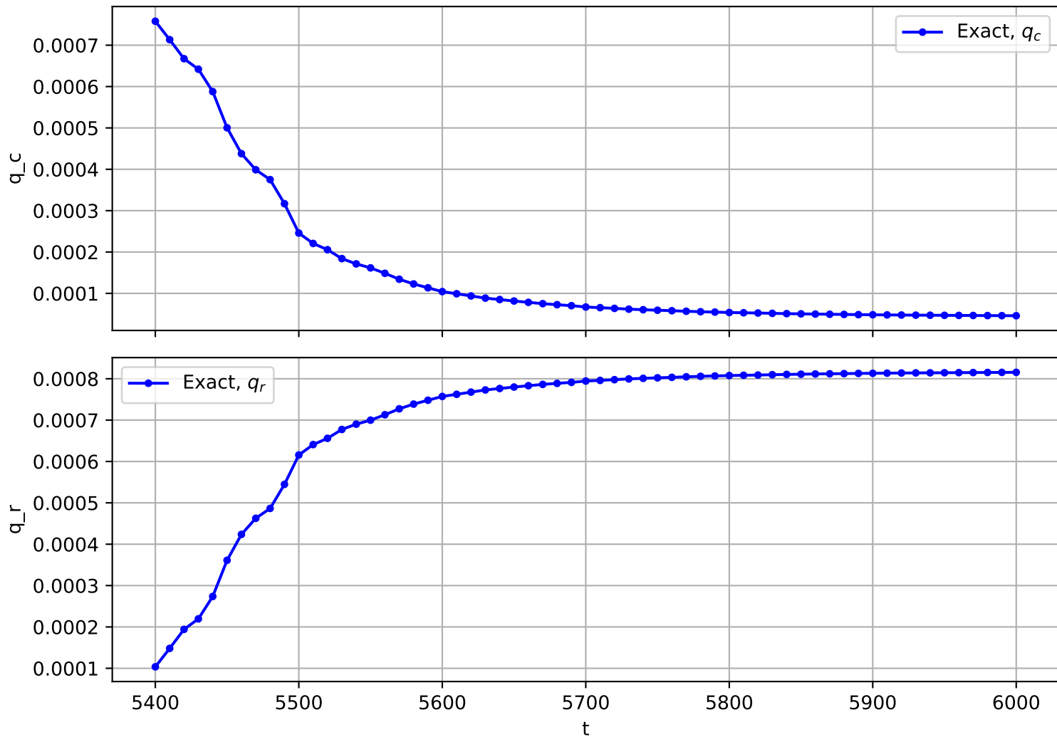
Trajectory No. 2391
