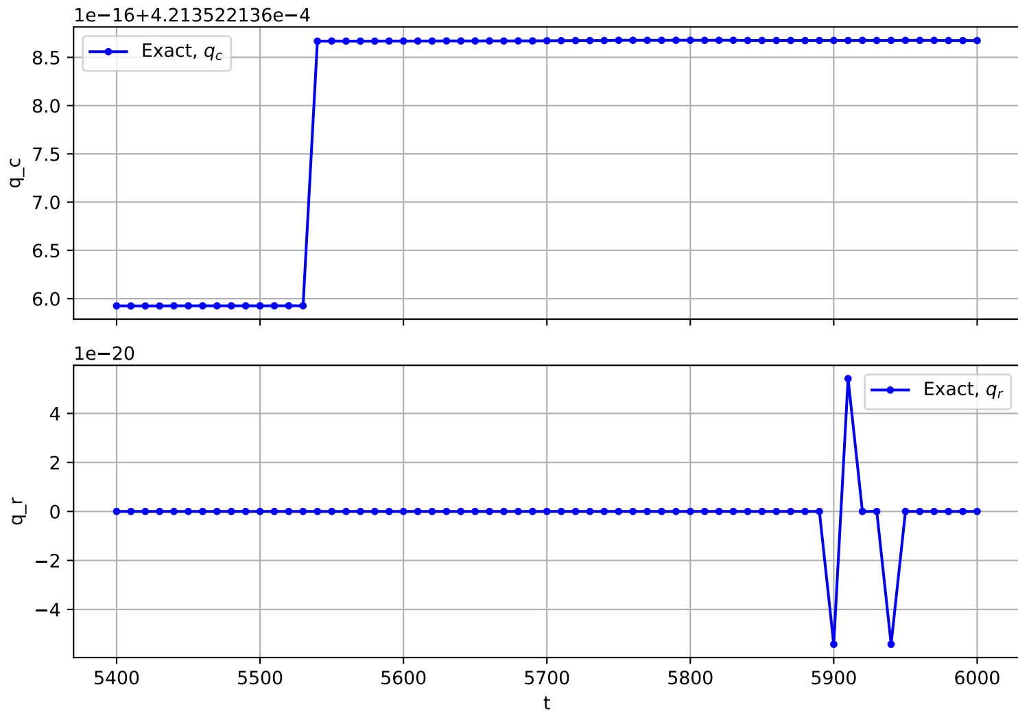
Trajectory No. 2401
