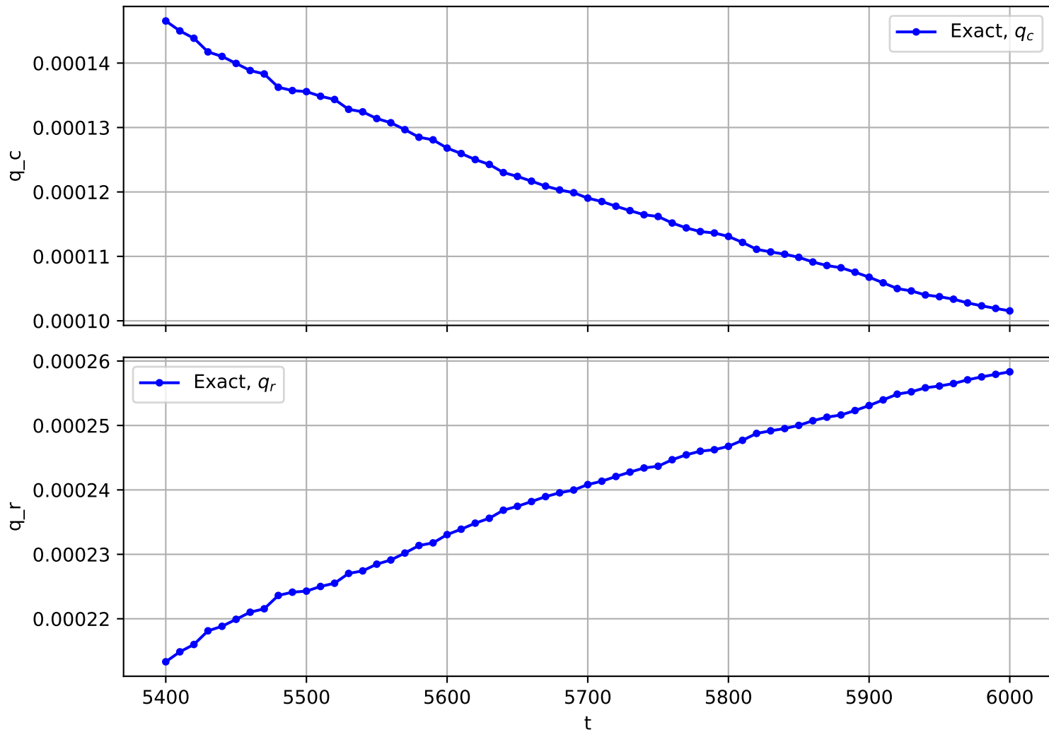
Trajectory No. 2489
