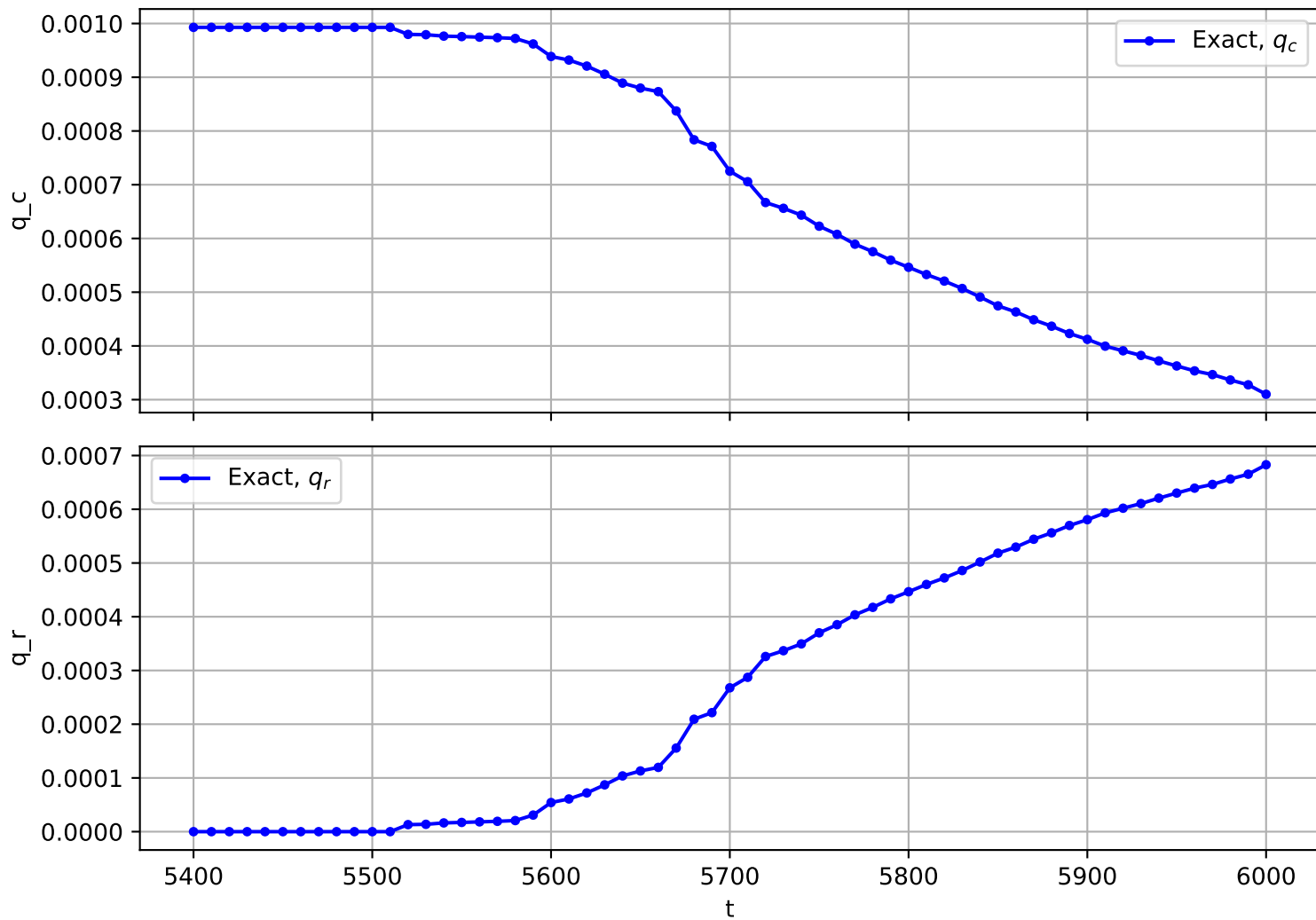
Trajectory No. 2499
