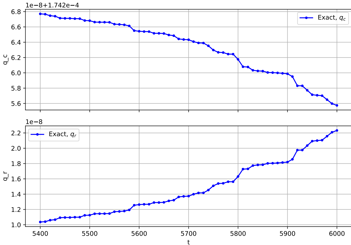
Trajectory No. 2534
