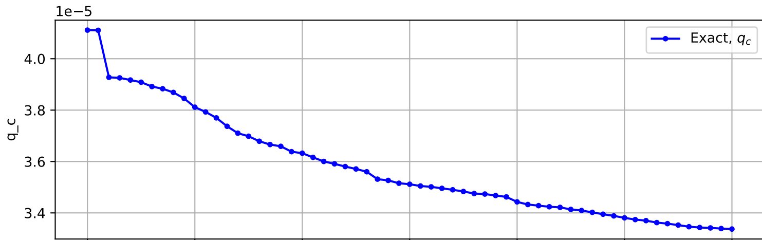
Trajectory No. 255
