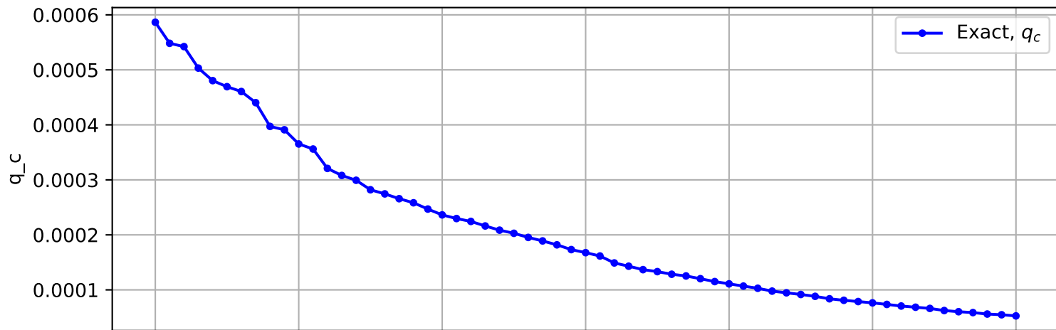
Trajectory No. 2580
