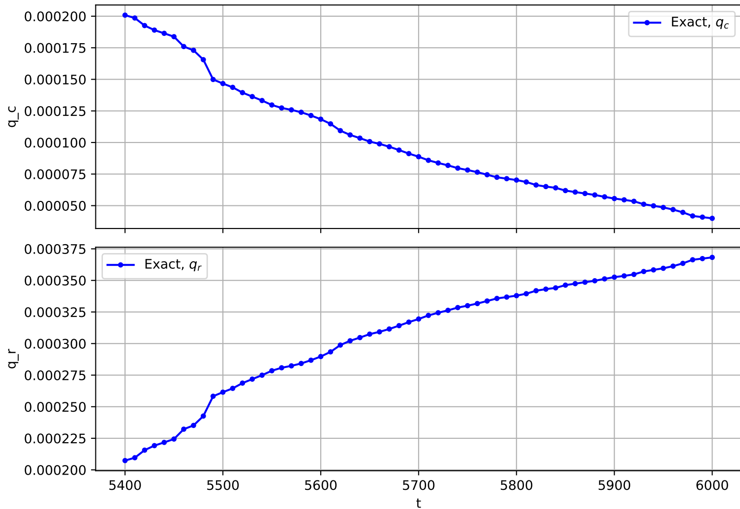
Trajectory No. 2585
