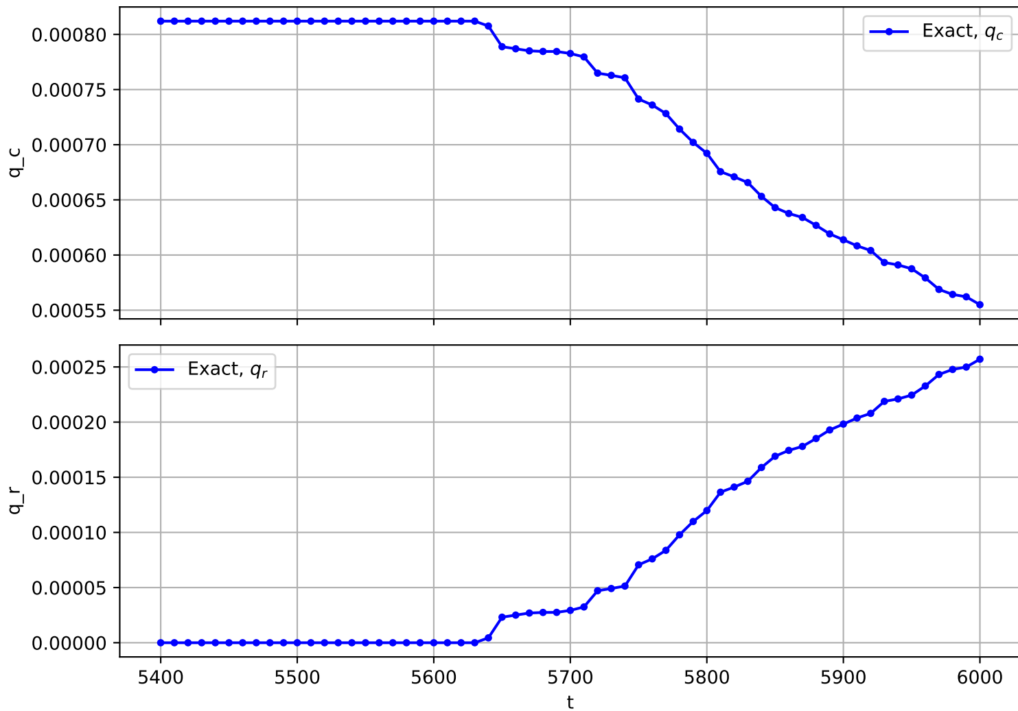
Trajectory No. 2626
