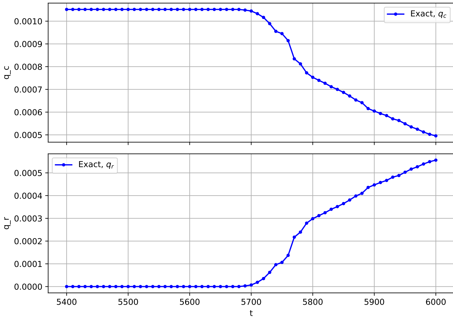
Trajectory No. 2635
