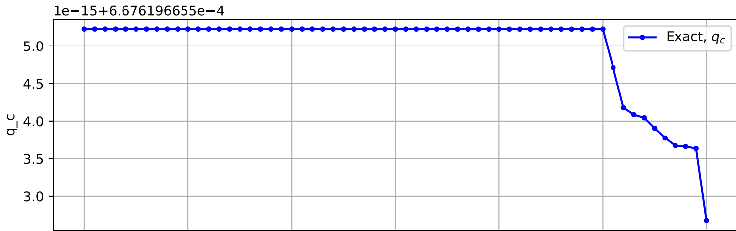
Trajectory No. 2649
