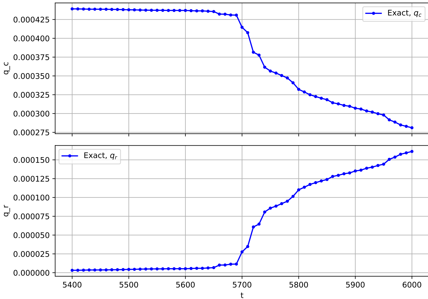
Trajectory No. 2663
