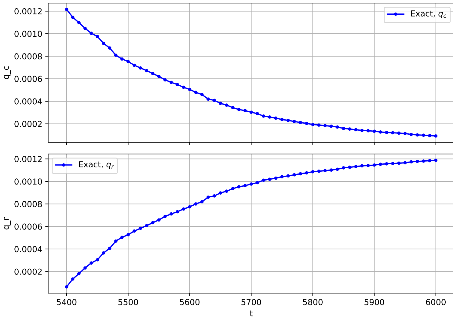
Trajectory No. 2665
