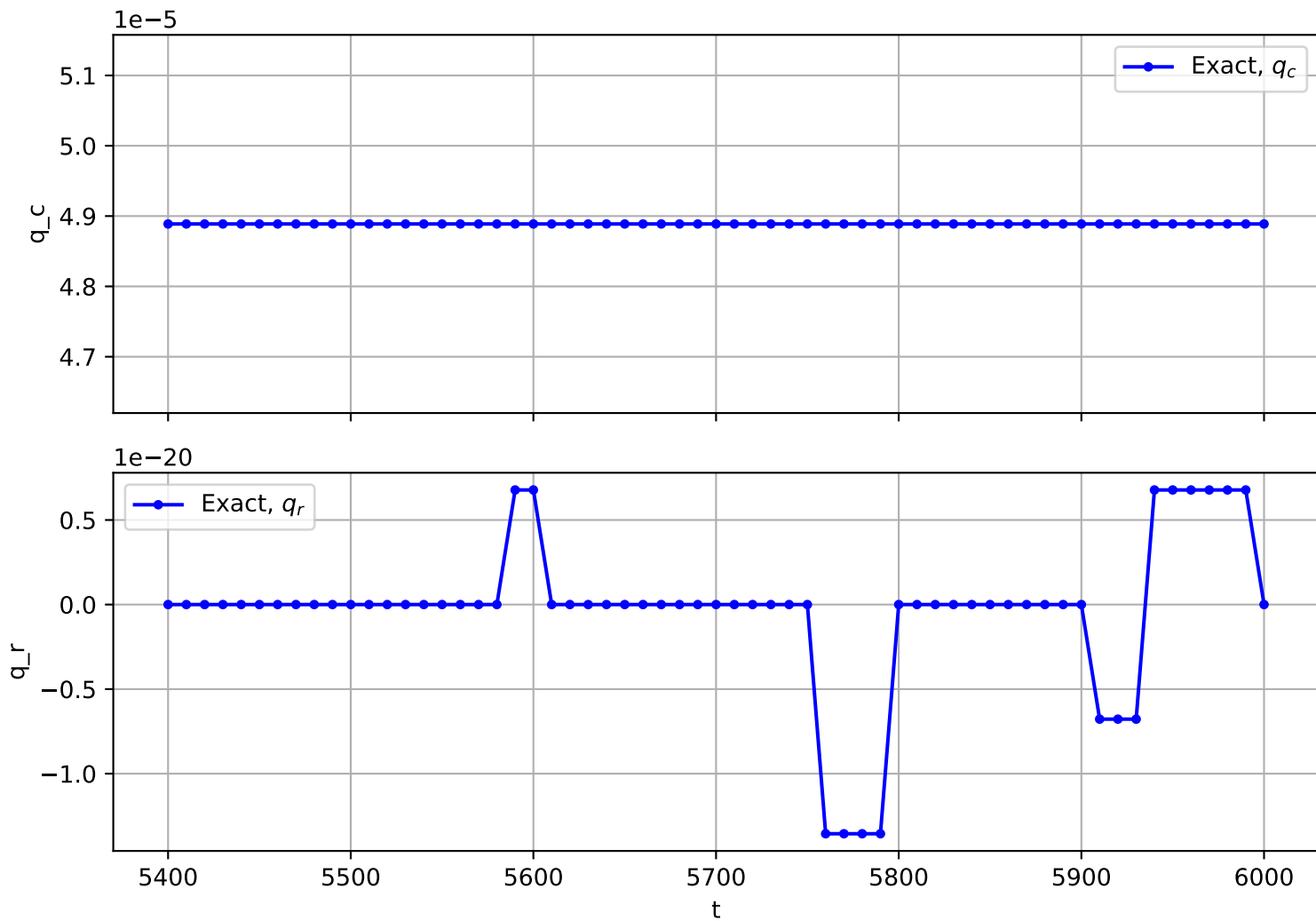
Trajectory No. 267
