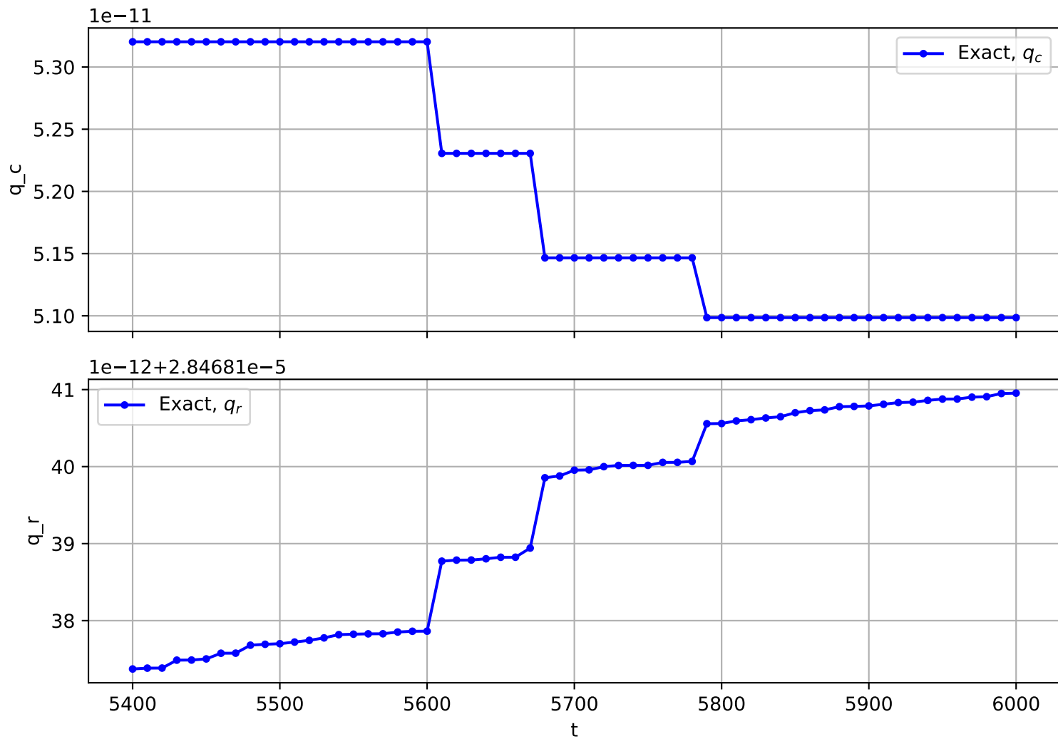
Trajectory No. 2674
