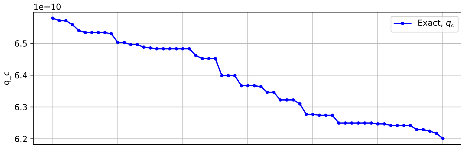
Trajectory No. 2676
