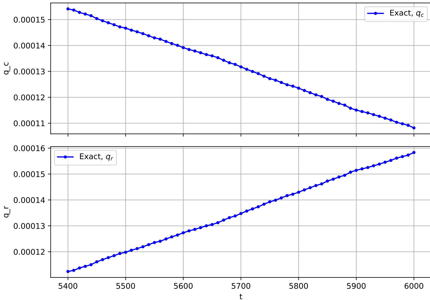
Trajectory No. 2678
