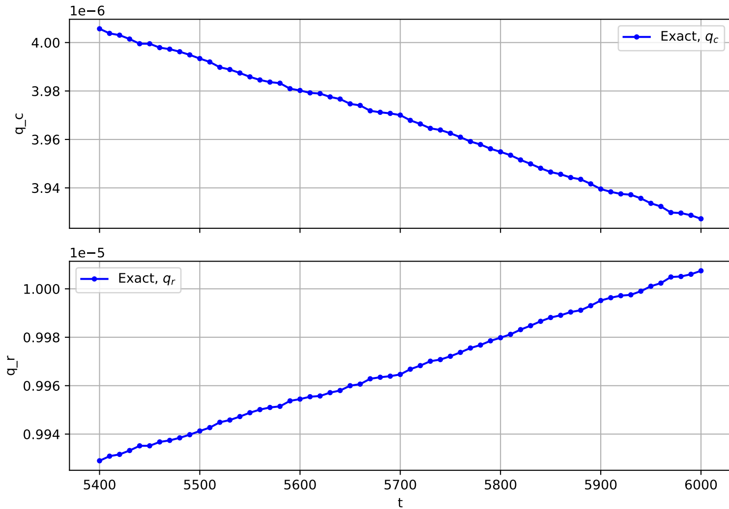
Trajectory No. 269
