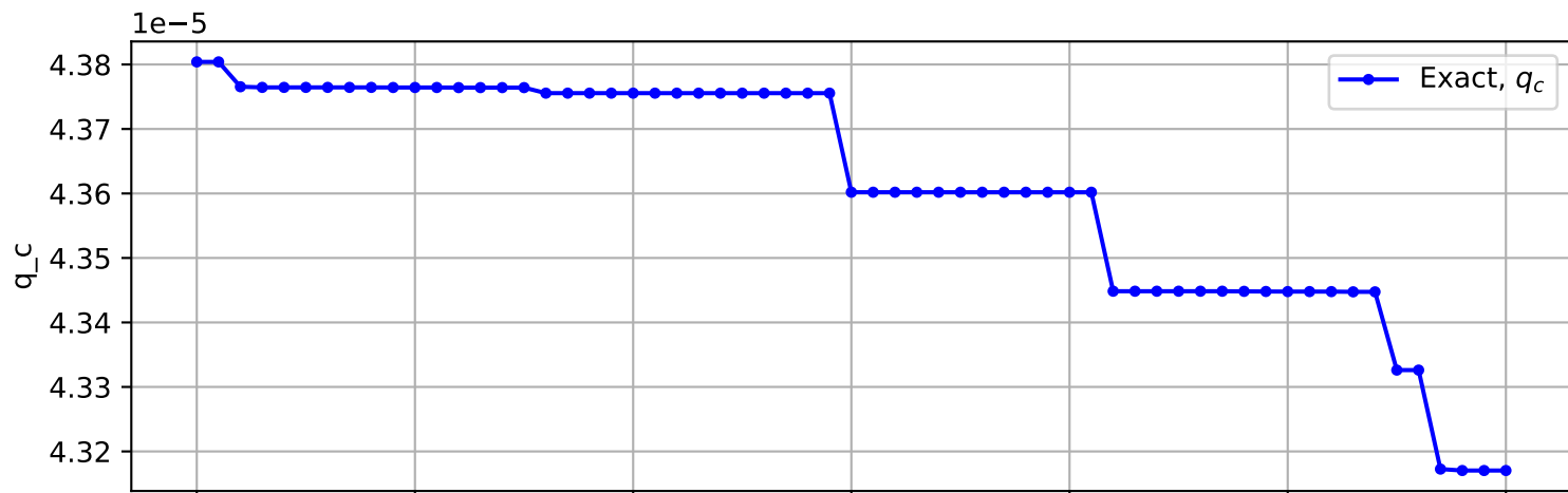
Trajectory No. 27
