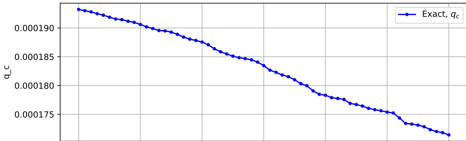
Trajectory No. 270
