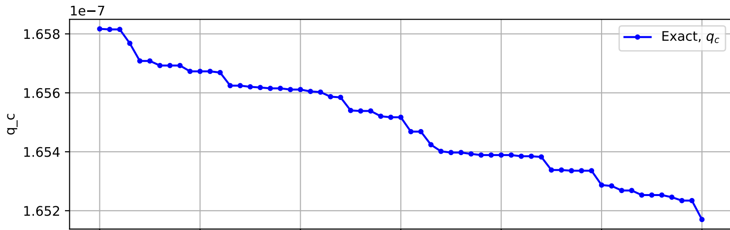
Trajectory No. 2705
