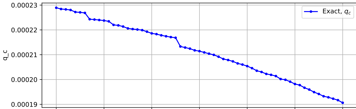
Trajectory No. 2712
