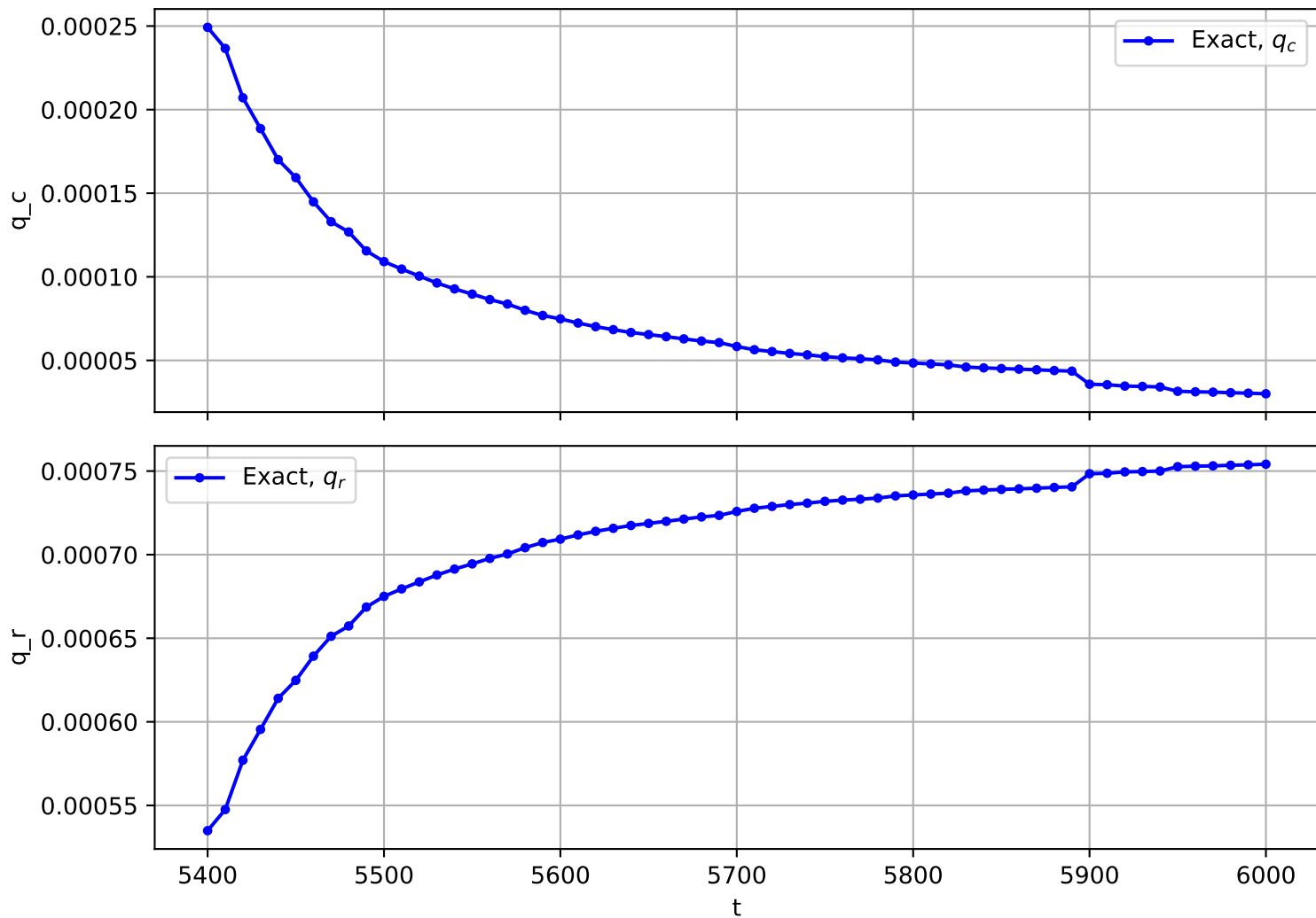
Trajectory No. 2734
