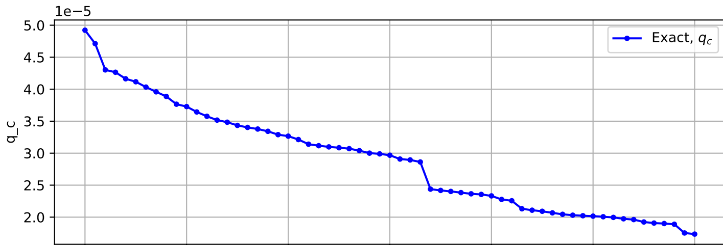
Trajectory No. 2740
