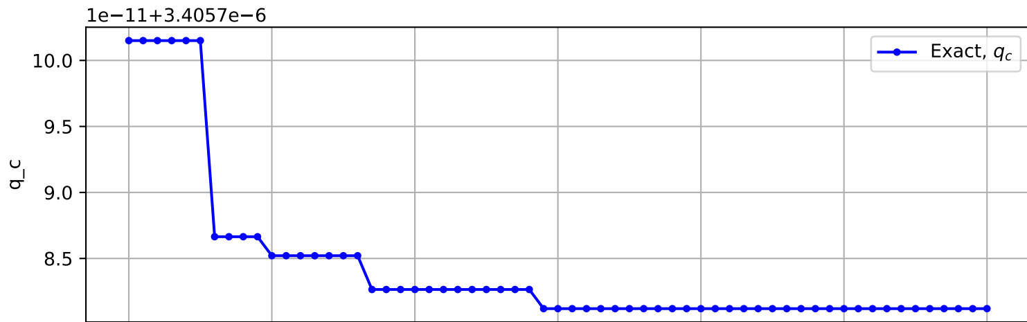
Trajectory No. 2747
