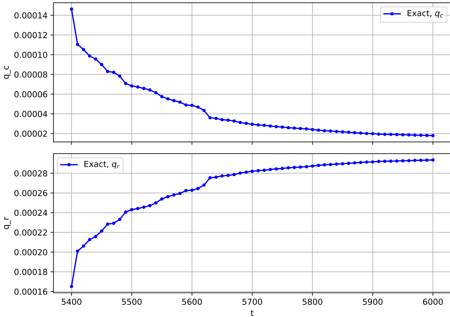
Trajectory No. 2769
