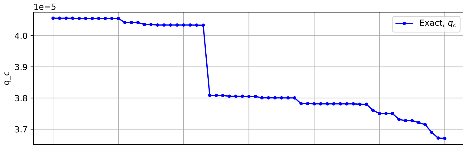
Trajectory No. 2794
