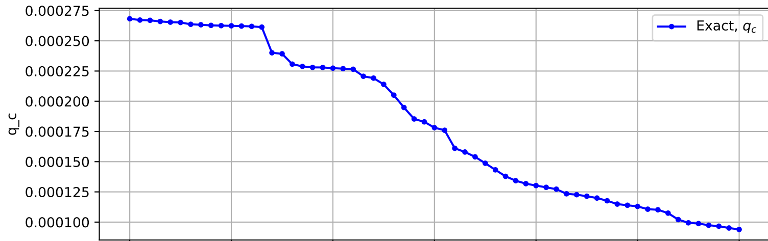
Trajectory No. 2799
