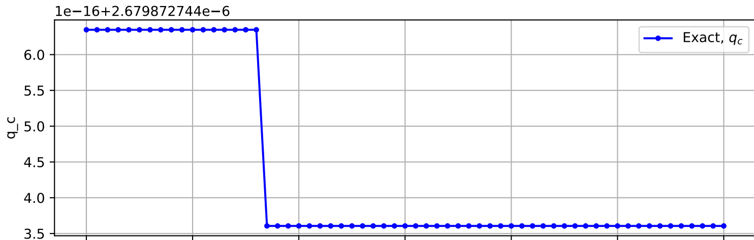
Trajectory No. 2824
