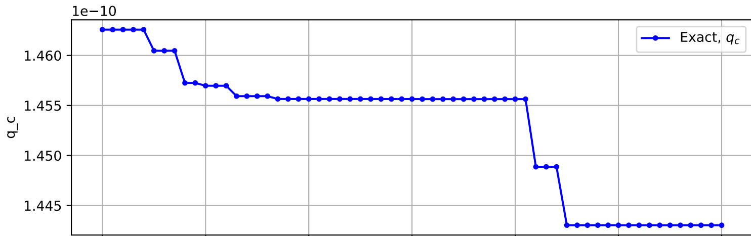
Trajectory No. 2828
