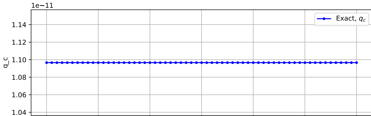
Trajectory No. 2845
