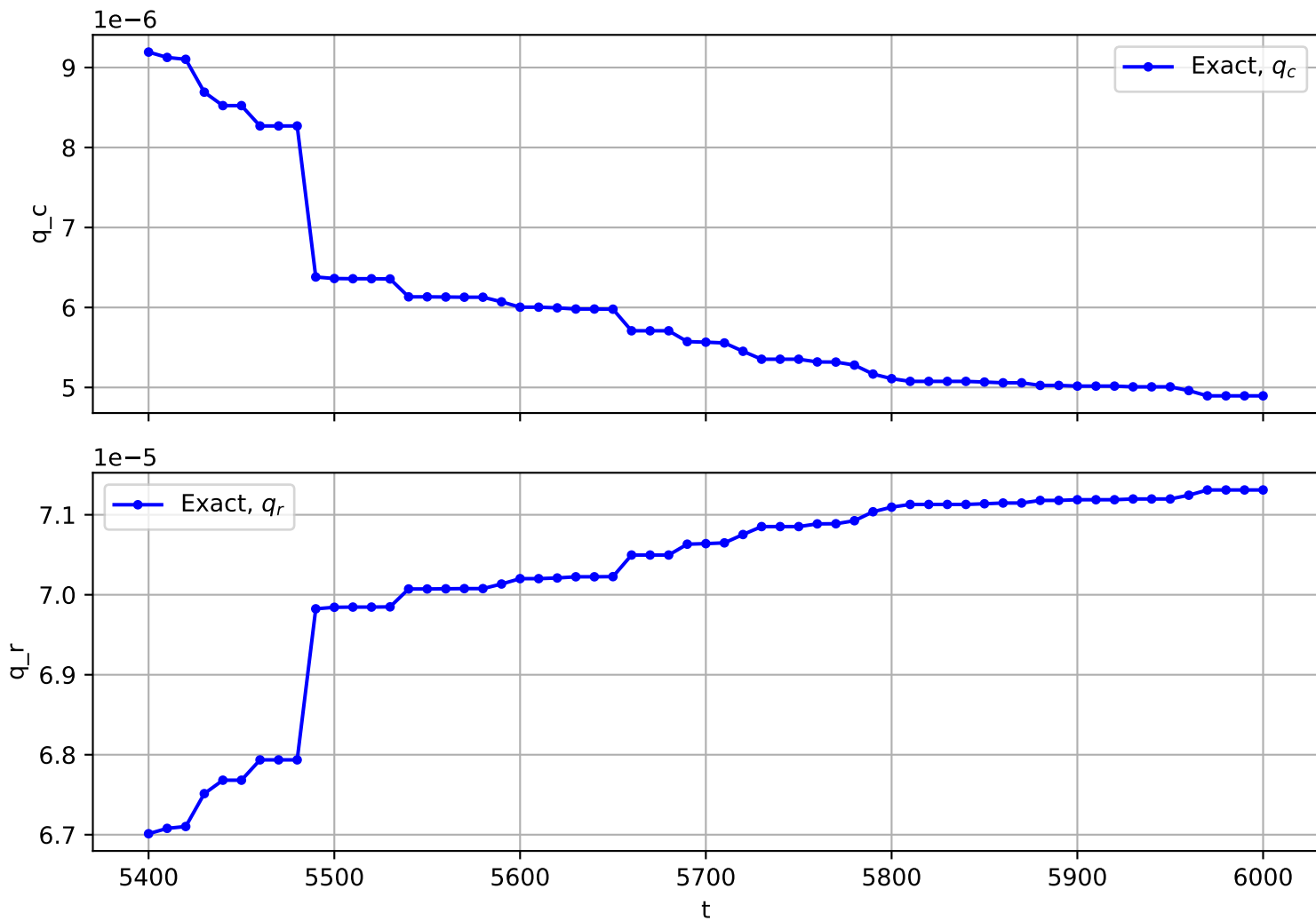
Trajectory No. 2879
