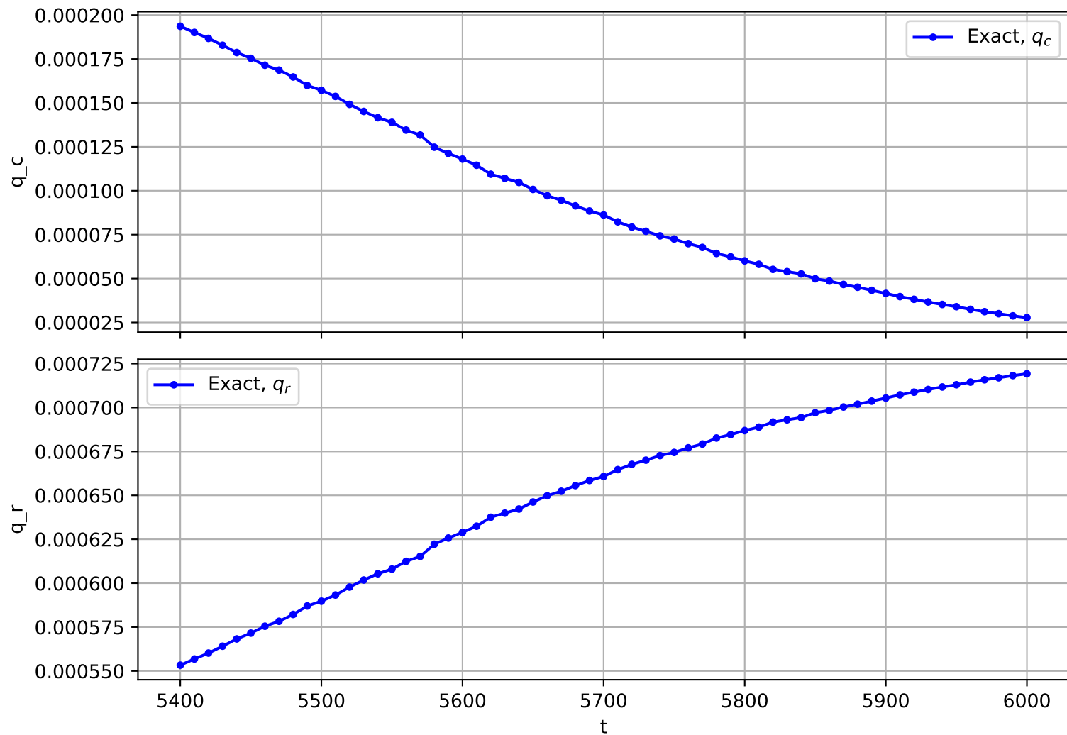
Trajectory No. 2883
