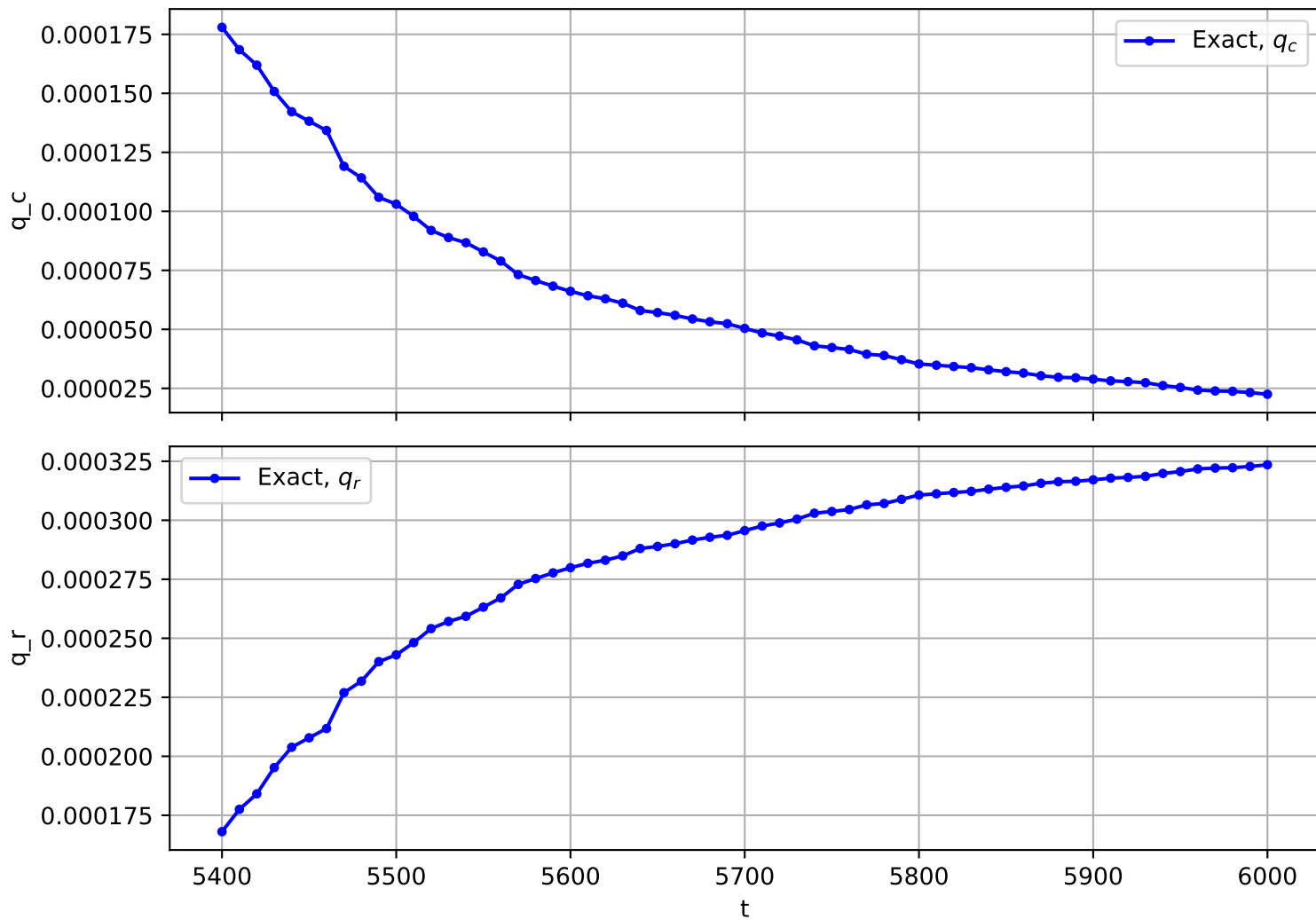
Trajectory No. 2887
