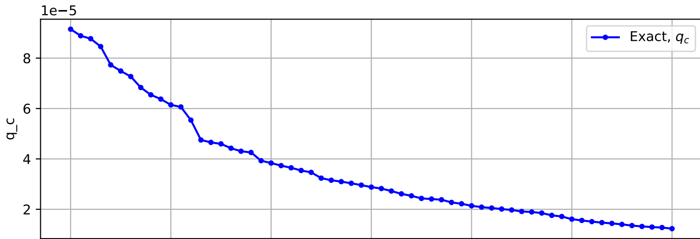
Trajectory No. 2892
