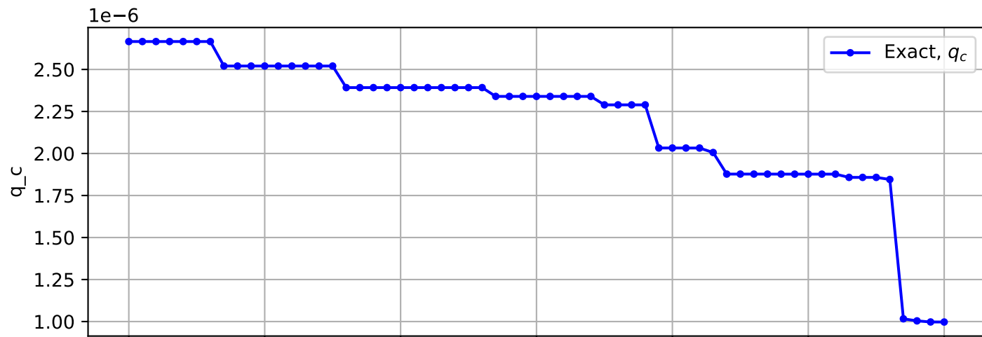
Trajectory No. 2897
