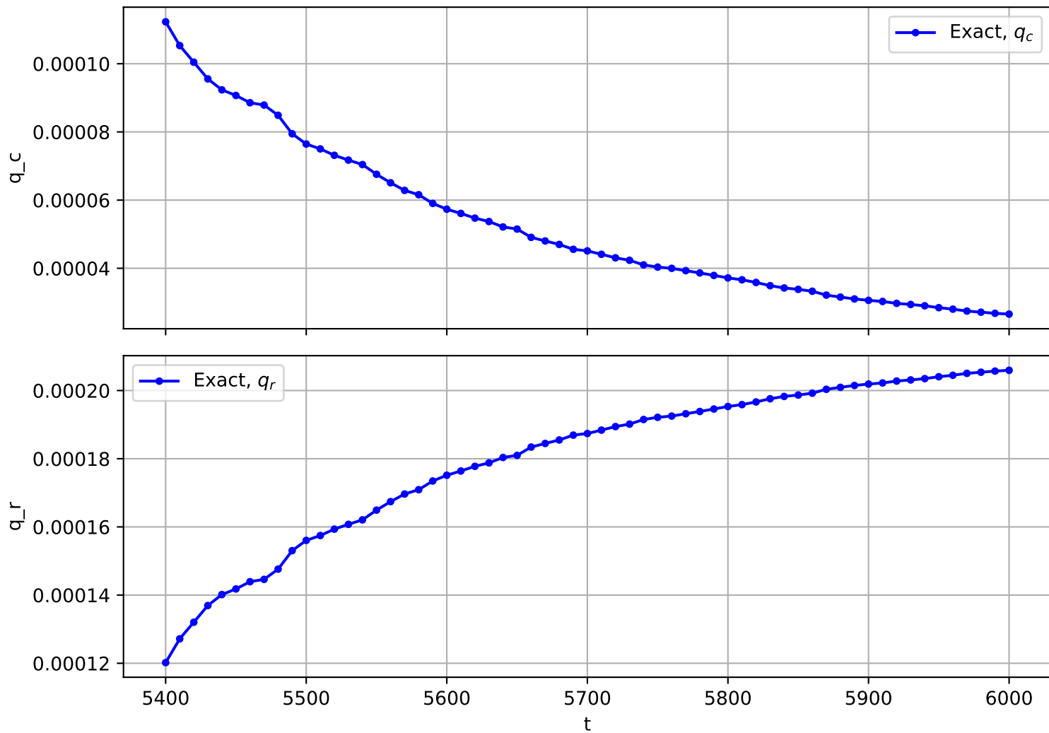
Trajectory No. 2906
