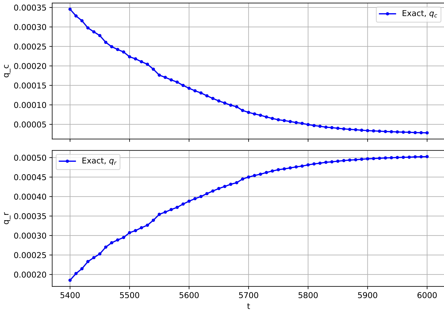
Trajectory No. 2930
