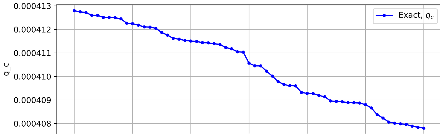
Trajectory No. 2934
