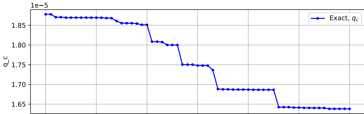
Trajectory No. 2955
