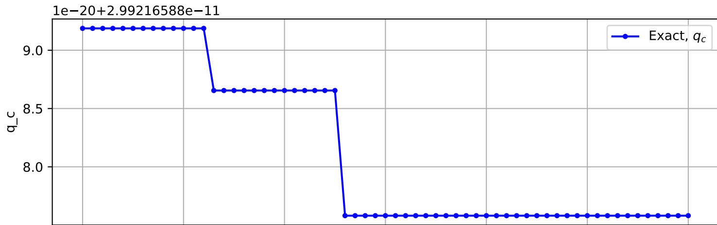
Trajectory No. 2979
