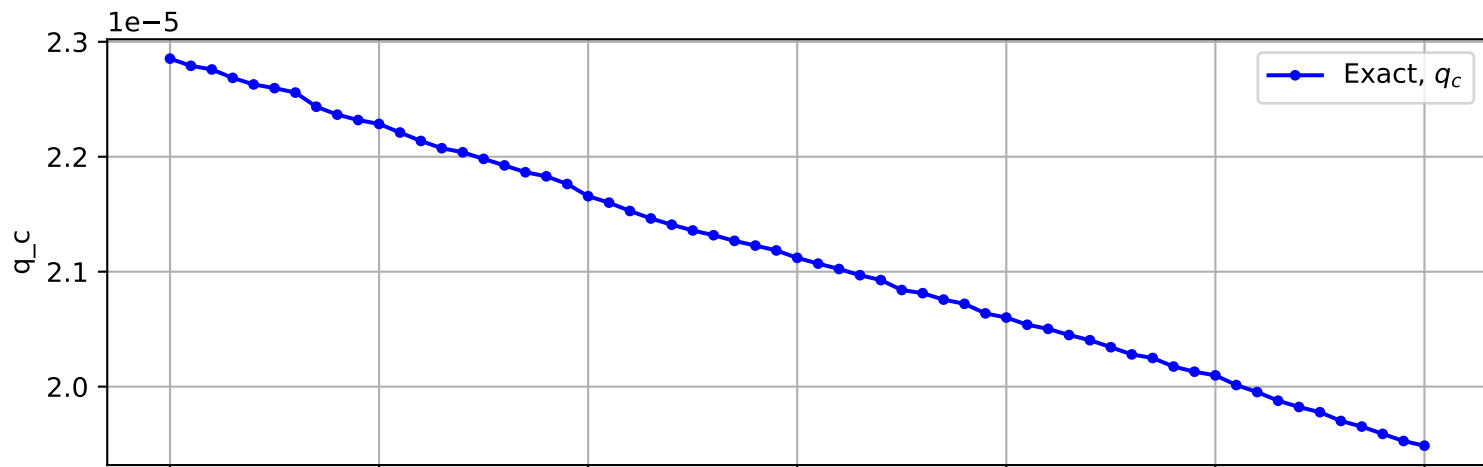
Trajectory No. 2983
