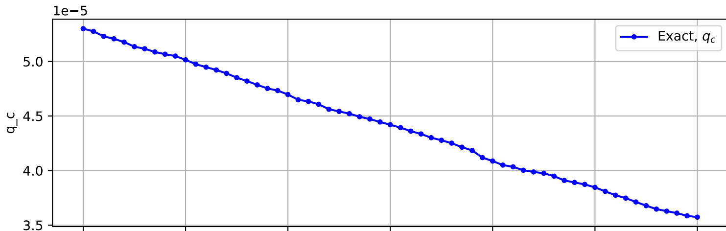
Trajectory No. 2984
