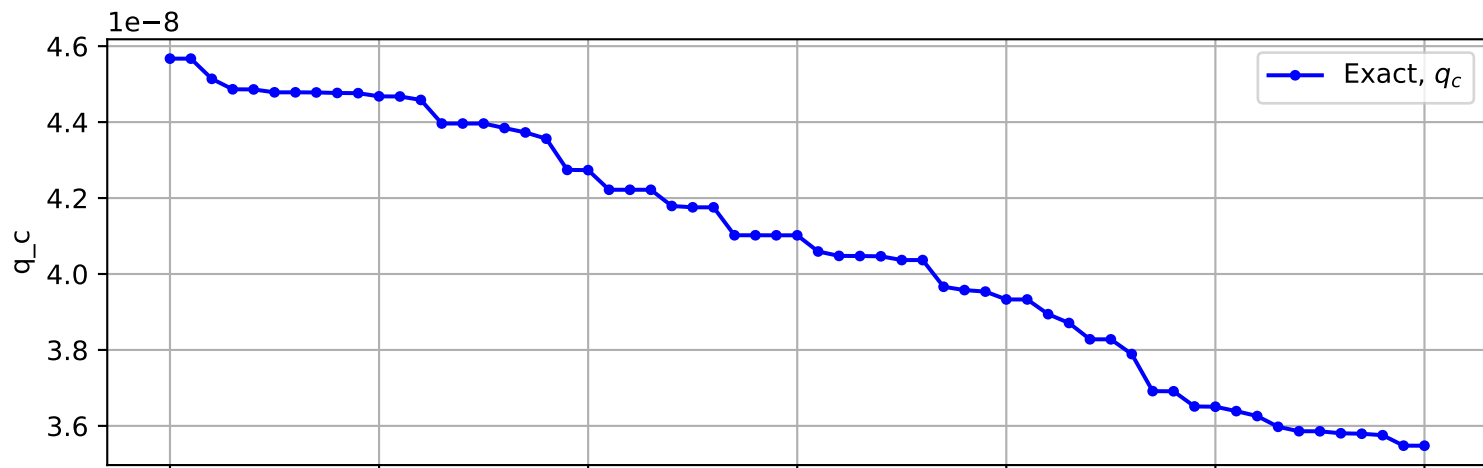
Trajectory No. 3011
