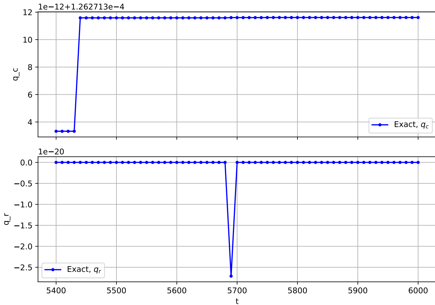
Trajectory No. 302
