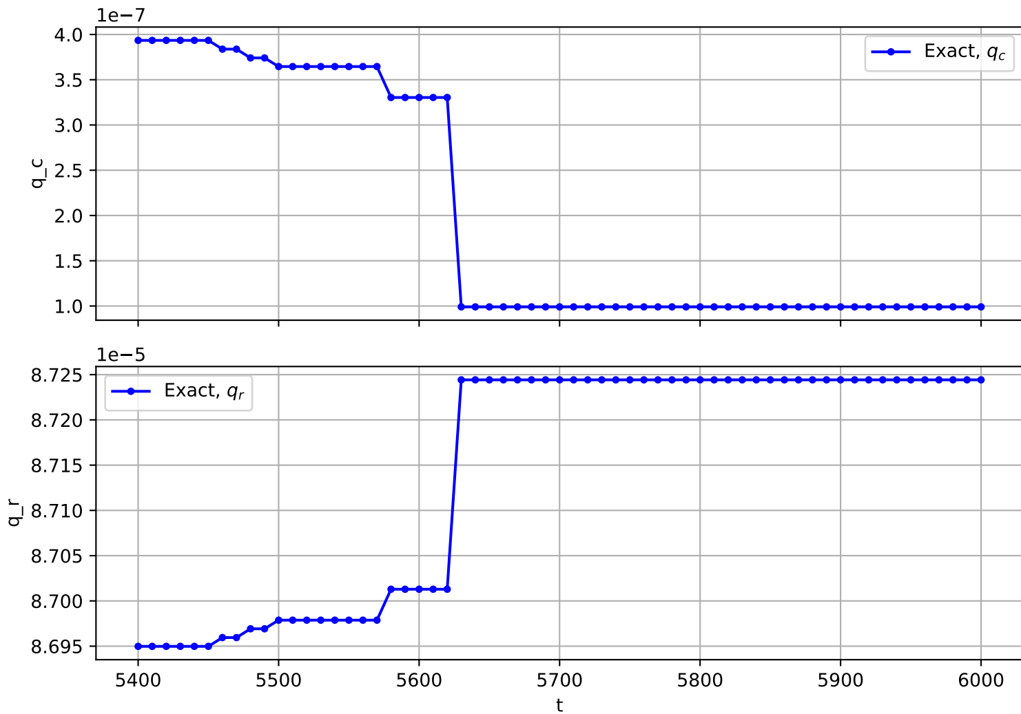
Trajectory No. 3092
