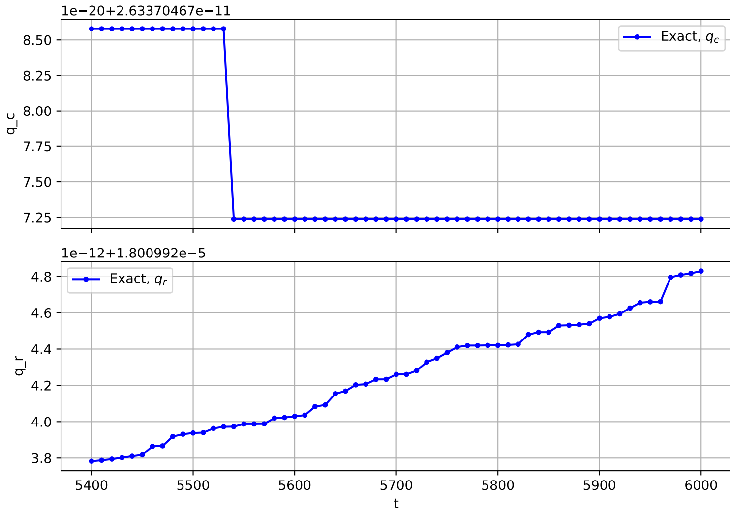
Trajectory No. 3096
