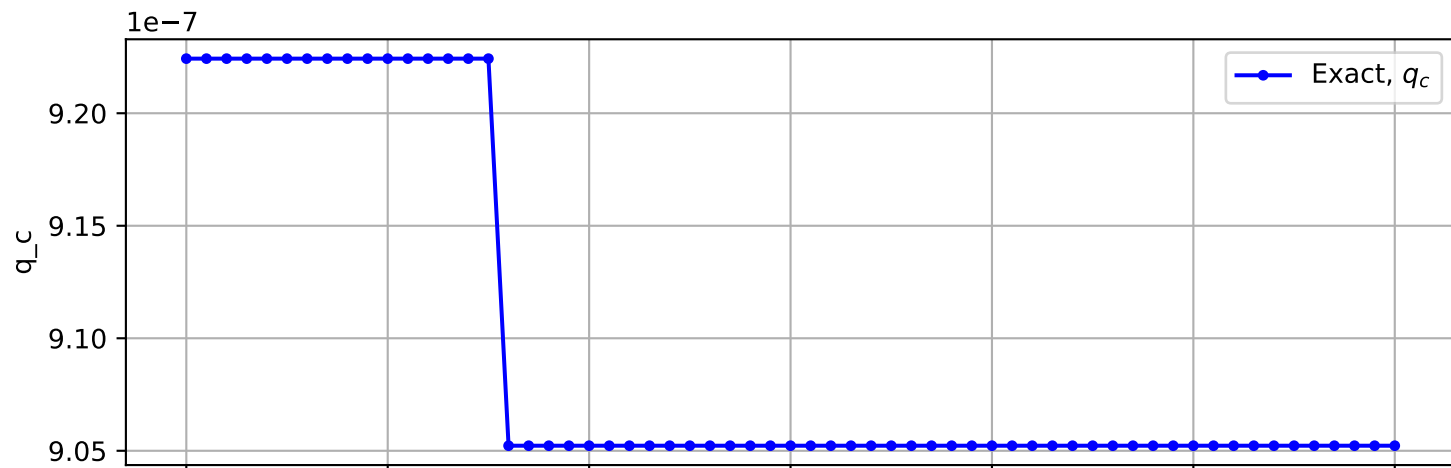
Trajectory No. 3142
