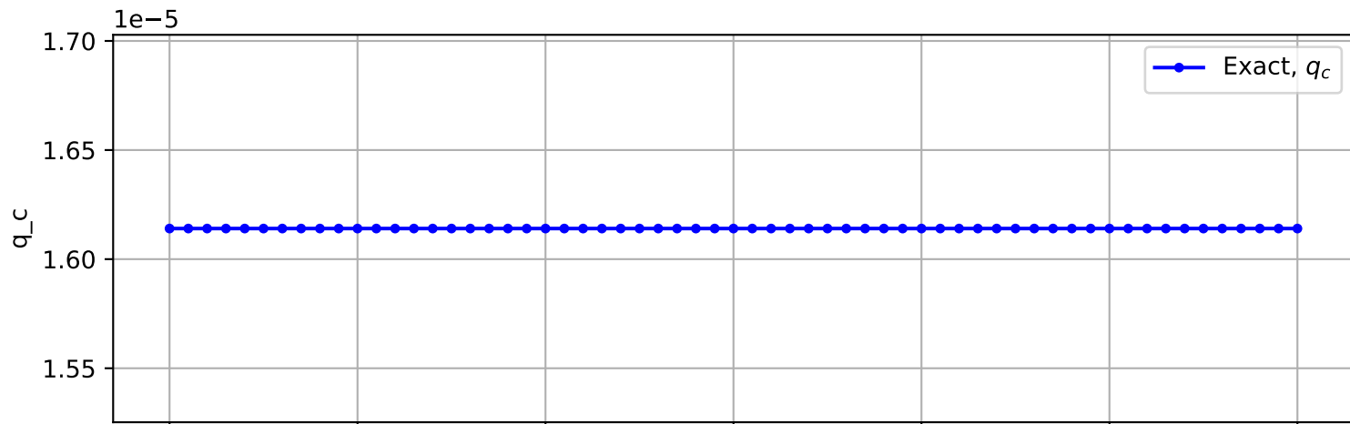
Trajectory No. 3161
